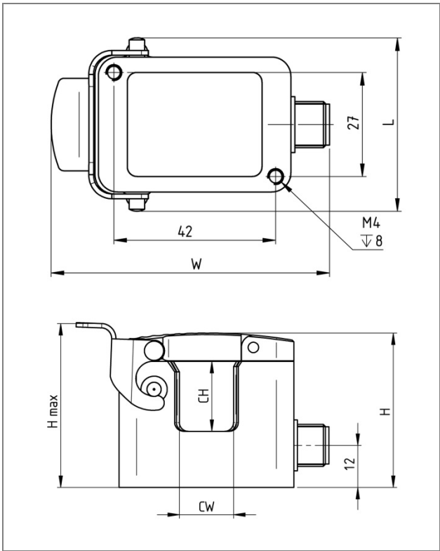
Sensor design with hinged cover
