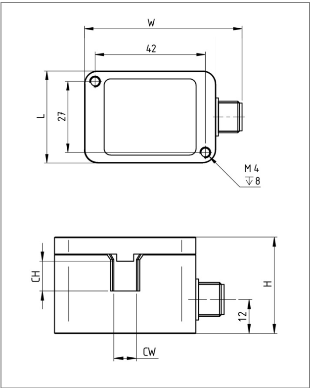
Sensor design with screw cover
