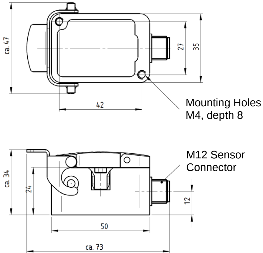
Figure 5: Drawing of sensor model S.
